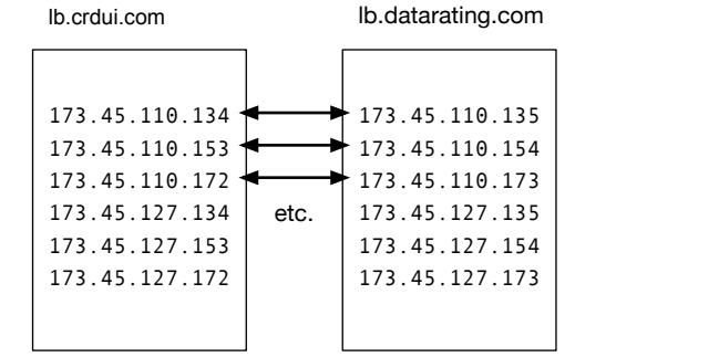
(a) Neighboring relationships of IPs between seemingly unrelated domains used for monitoring.
